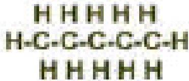
Straight chain (pentane) C_5H_{12}
